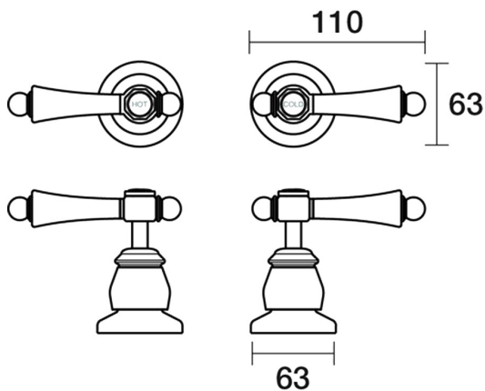
Tudor Top Assemblies Wall Pair Porcelain Lever Ceramic Disc B31.082.4.06 - Chrome / Sienna Red
