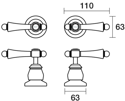
Tudor Top Assemblies Wall Pair Porcelain Lever Ceramic Disc B31.082.4.12 - 23k Brushed Gold
