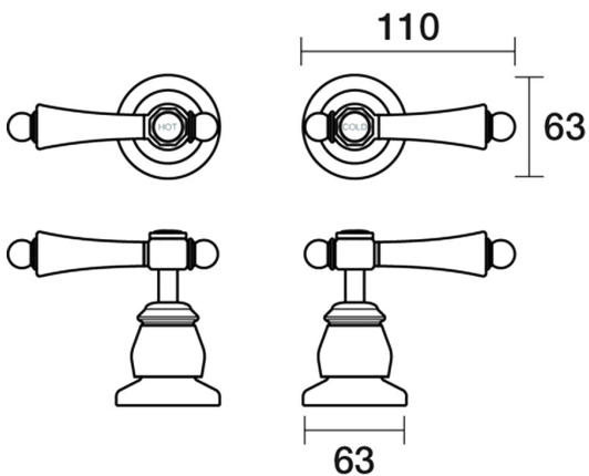
Tudor Top Assemblies Wall Pair Porcelain Lever Ceramic Disc B31.082.4.17 - Gold / Victorian Green
