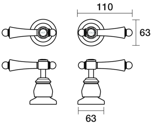
Tudor Top Assemblies Wall Pair Porcelain Lever Ceramic Disc B31.082.4.40 - Rumbled Brass
