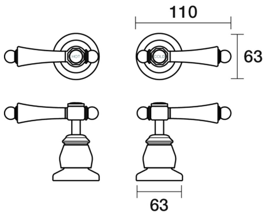
Tudor Top Assemblies Wall Pair Porcelain Lever Ceramic Disc B31.082.4.41 - Brushed Brass
