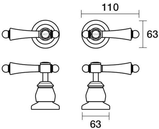
Tudor Top Assemblies Wall Pair Porcelain Lever Ceramic Disc B31.082.4.57 - Matt Nickel
