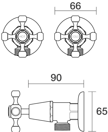
Tudor Washing Machine Stops Wall Pair B31.091.1.01 - Chrome
