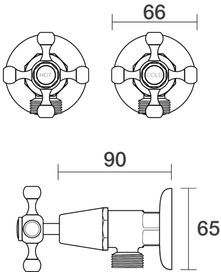
Tudor Washing Machine Stops Wall Pair B31.091.1.40 - Rumbled Brass
