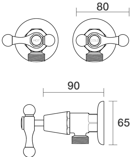
Tudor Washing Machine Stops Wall Pair Lever Ceramic Disc B31.091.3.03 - Chrome / White
