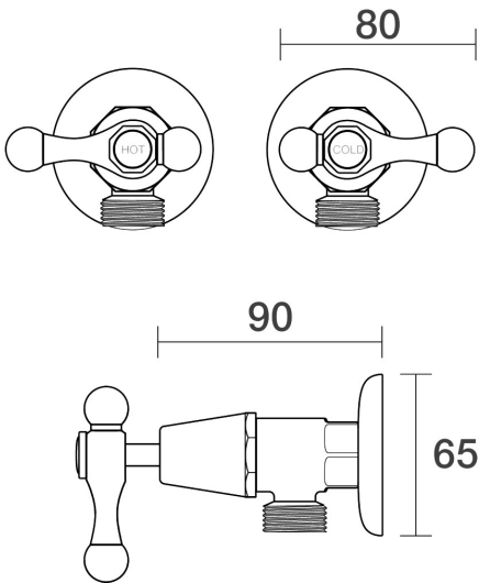
Tudor Washing Machine Stops Wall Pair Lever Ceramic Disc B31.091.3.15 - Gold / Apricot
