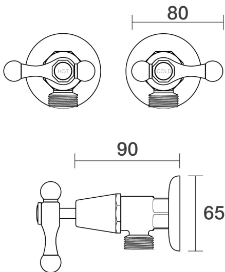
Tudor Washing Machine Stops Wall Pair Lever Ceramic Disc B31.091.3.57 - Matt Nickel
