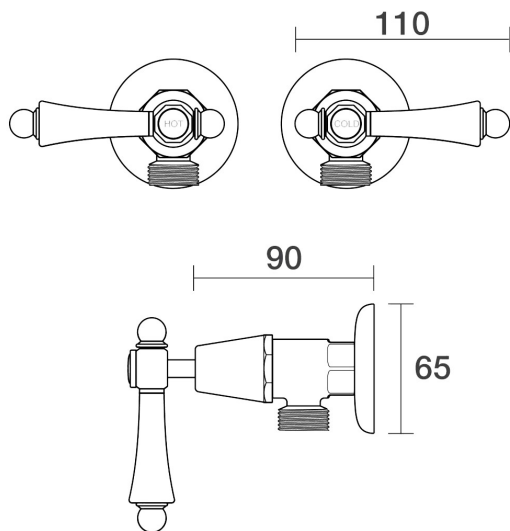
Tudor Washing Machine Stops Wall Pair Porcelain Lever Ceramic Disc B31.091.4.13 - Gold / White
