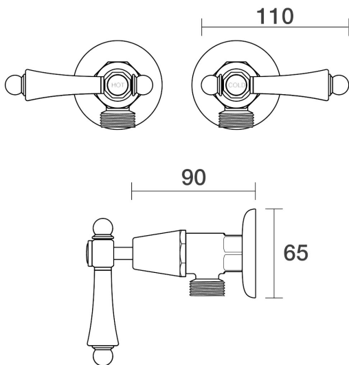
Tudor Washing Machine Stops Wall Pair Porcelain Lever Ceramic Disc B31.091.4.21 - Brushed Rose Gold
