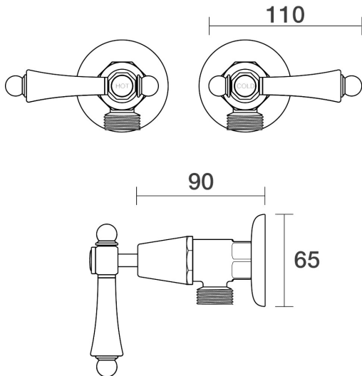
Tudor Washing Machine Stops Wall Pair Porcelain Lever Ceramic Disc B31.091.4.54 - Volcanic Grey
