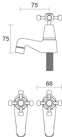
Tudor Pillar Taps Pair Ceramic Disc B31.111.2.45 - Native Brass
