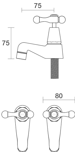
Tudor Pillar Taps Pair Lever Ceramic Disc B31.111.3.27 - Satin Pearl
