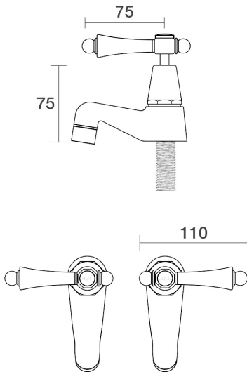
Tudor Pillar Taps Pair Porcelain Lever Ceramic Dia: 111.4.16 - Gold / Sienna Red
