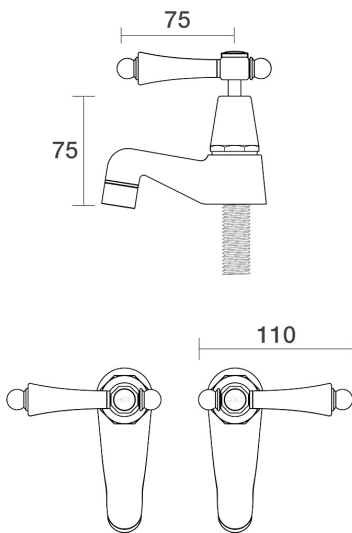
Tudor Pillar Taps Pair Porcelain Lever Ceramic Disc 111.4.23 - Gunmetal
