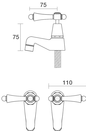
Tudor Pillar Taps Pair Porcelain Lever Ceramic Disc Part 111.4.25 - Brushed Nickel
