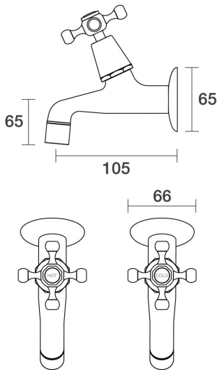
Tudor Female Bibs Wall Pair Ceramic Disc B31.121.2.01 - Chrome
