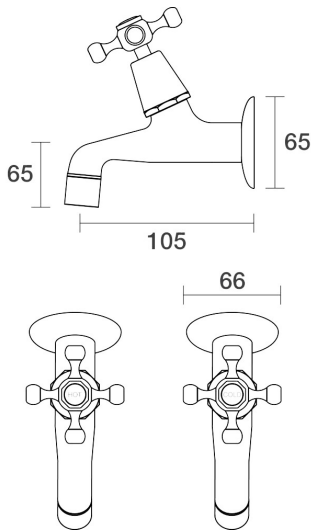
Tudor Female Bibs Wall Pair Ceramic Disc B31.121.2.23 - Gunmetal
