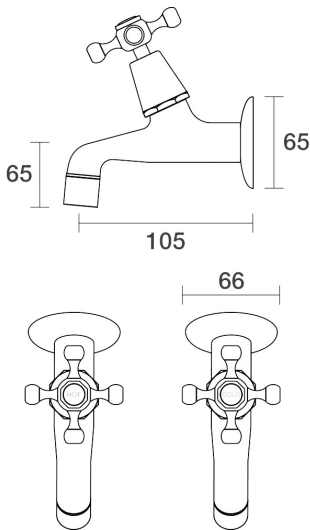
Tudor Female Bibs Wall Pair Ceramic Disc B31.121.2.40 - Rumbled Brass
