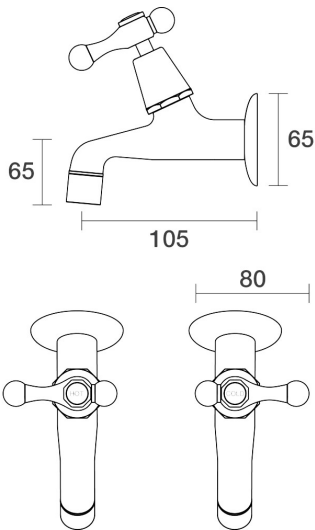
Tudor Female Bibs Wall Pair Lever Ceramic Disc B31.121.3.21 - Brushed Rose Gold
