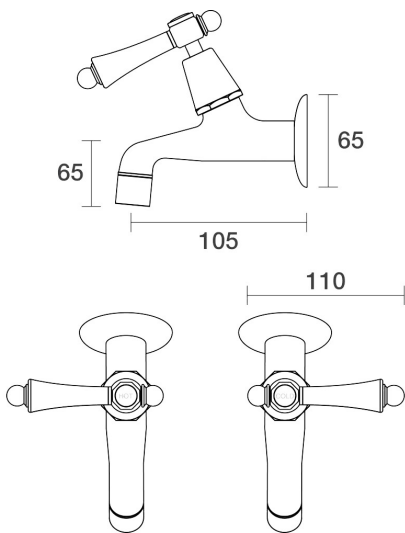
Tudor Female Bibs Wall Pair Porcelain Lever Ceramic Disc B31.121.4.02 - Brushed Chrome
