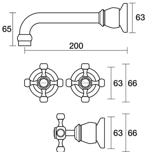
Tudor Wall Basin Set 200mm Outlet Ceramic Disc B31.152.2.12 - 23k Brushed Gold
