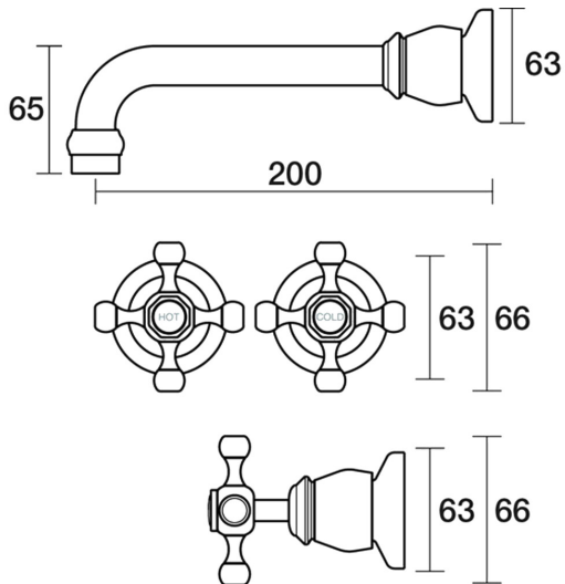
Tudor Wall Basin Set 200mm Outlet Ceramic Disc B31.152.2.54 - Volcanic Grey
