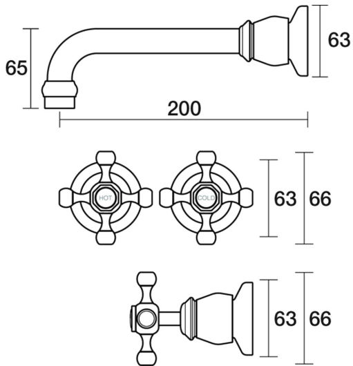
Tudor Wall Basin Set 200mm Outlet Ceramic Disc B31.152.2.67 - Vintage Brass
