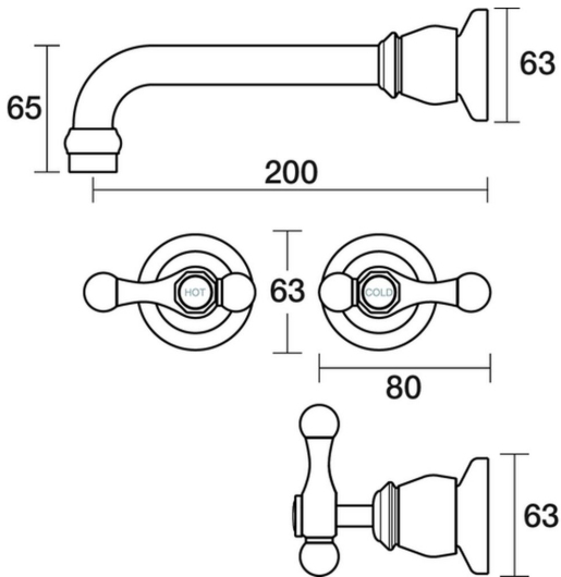
Tudor Wall Basin Set 200mm Outlet Lever Ceramic Disc B31.152.3.01 - Chrome
