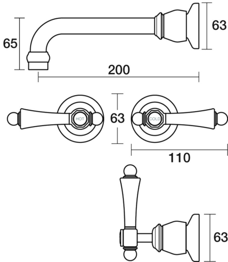
Tudor Wall Basin Set 200mm Outlet Porcelain Lever Ceramic Disc B31.152.4.32 - Midnight Black
