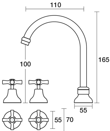
Bell Basin Set Swivel B32.011.1.11 - 23k Gold
