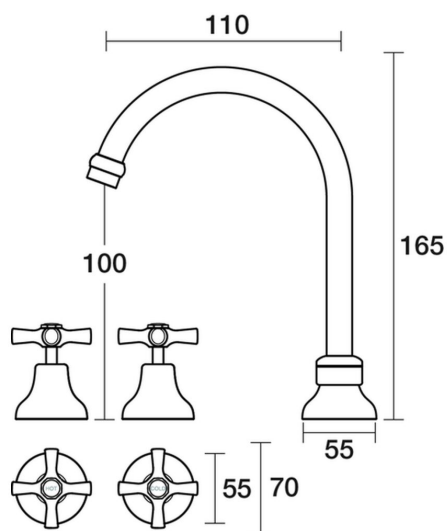
Bell Basin Set Swivel Ceramic Disc B32.011.2.01 - Chrome
