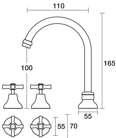
Bell Basin Set Swivel Ceramic Disc B32.011.2.17 - Gold / Victorian Green
