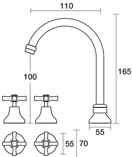
Bell Basin Set Swivel Ceramic Disc B32.011.2.19 - 23k Brushed Brass Gold
