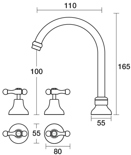
Bell Basin Set Swivel Lever Ceramic Disc B32.011.3.03 - Chrome / White
