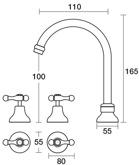
Bell Basin Set Swivel Lever Ceramic Disc B32.011.3.11 - 23k Gold
