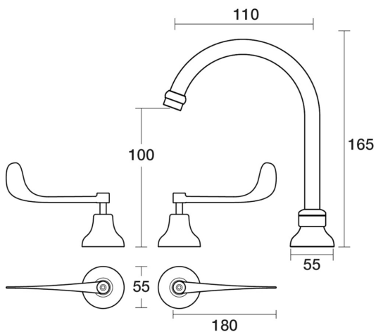
Bell Basin Set Swivel DDA Compliant Extended Lever Ceramic Disc B32.011.5.05 - Chrome / Apricot
