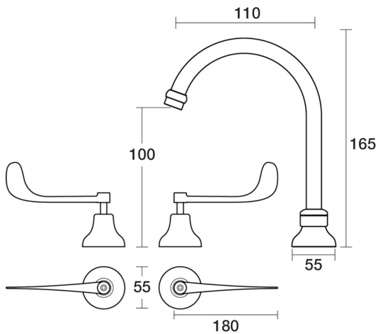
Bell Basin Set Swivel DDA Compliant Extended Lever Ceramic Disc B32.011.5.14 - Gold / Ivory
