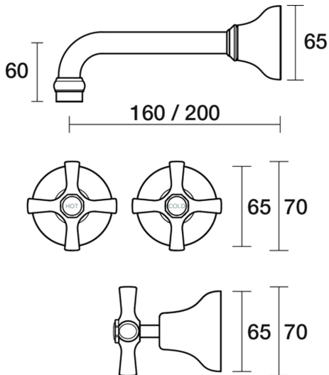
Bell Wall Bath Set 160mm Outlet Ceramic Disc B32.021.2.16 - Gold / Sienna Red
