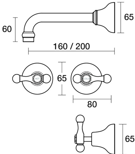
Bell Wall Bath Set 160mm Outlet Lever Ceramic Disc Dec 2021.3.01 - Chrome
