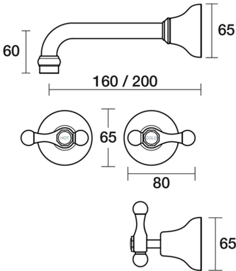
Bell Wall Bath Set 160mm Outlet Lever Ceramic Disc 2021.3.01 - Chrome
