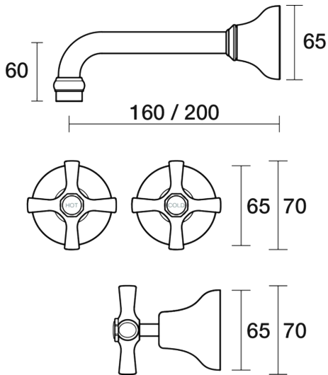
Bell Wall Bath Set 200mm Outlet Ceramic Disc B32.022.2.01 - Chrome
