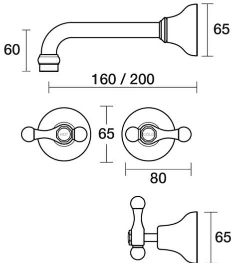
Bell Wall Bath Set 200mm Outlet Lever Ceramic Dec 2022.3.03 - Chrome / White
