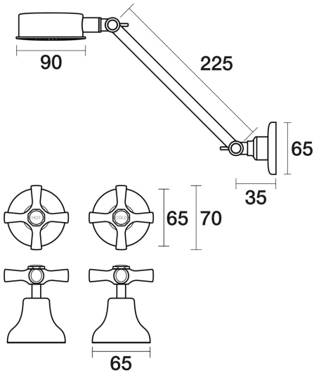
Bell Shower Set Adjustable Arm B32.031.1.01 - Chrome
