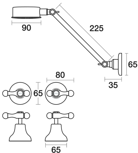
Bell Shower Set Adjustable Arm Lever Ceramic Disc Bell 2031.3.01 - Chrome
