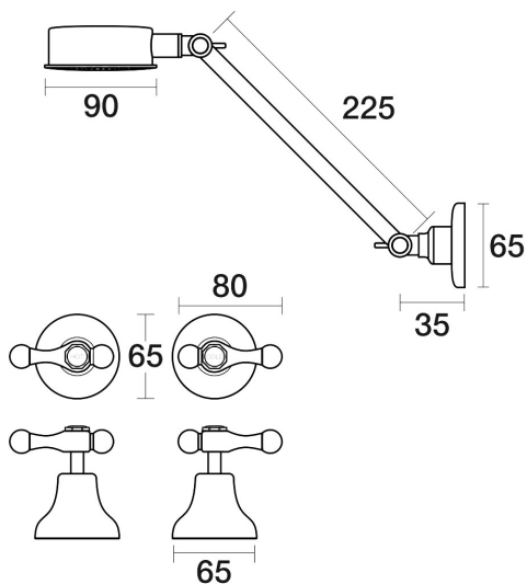
Bell Shower Set Adjustable Arm Lever Ceramic Disc Bell 031.3.10 - Chrome / Gold
