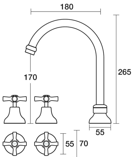
Bell Sink Set Hob Swivel Ceramic Disc B32.051.2.16 - Gold / Sienna Red
