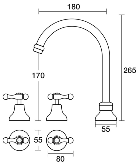
Bell Sink Set Hob Swivel Lever Ceramic Disc B32.051.3.14 - Gold / Ivory
