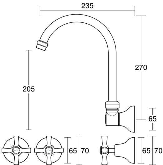
Bell Sink Set Wall Swivel Ceramic Disc B32.052.2.01 - Chrome
