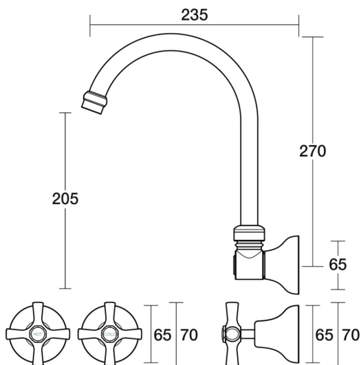
Bell Sink Set Wall Swivel Ceramic Disc B32.052.2.19 - 23k Brushed Brass Gold
