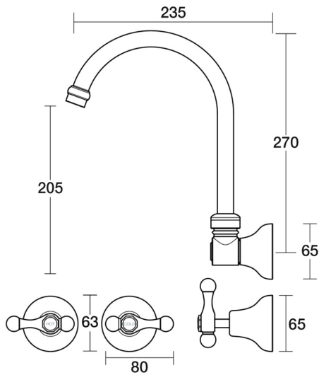
Bell Sink Set Wall Swivel Lever Ceramic Disc B32.052.3.06 - Chrome / Sienna Red
